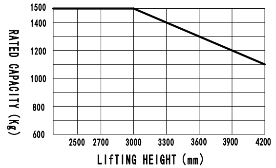
ES15-33DM RATED CAPACITIES GRAPH
